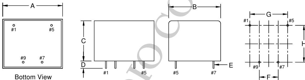
Bottom View
