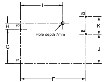
Footprint detail Top View
